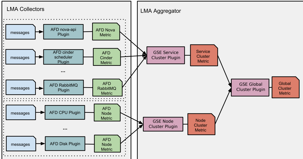
Fig. 5.1: Message flow for the AFD and GSE metrics
